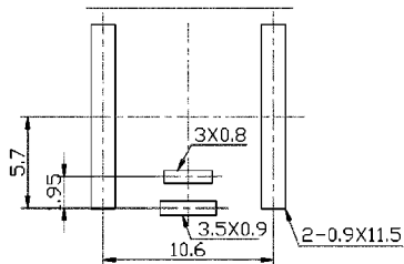
Dimensions of PC board holes (commend)
