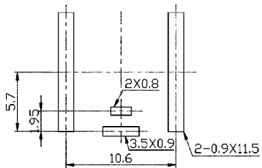
Dimensions of PC board holes (common)
