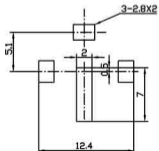
Dimensions of PC board holes (Commend)
