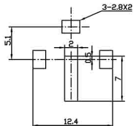
Dimensions of PC board holes (Commend)
