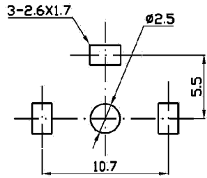
Dimensions of PC board holes (Commend)
