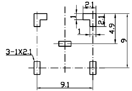
Dimensions of PC board holes (Commend)
