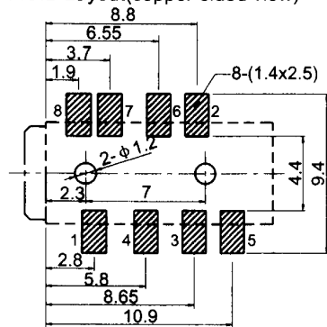
P.C.B Layout(copper-sided view)
