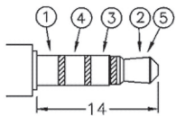
Ø3.5 MATE PLUG
