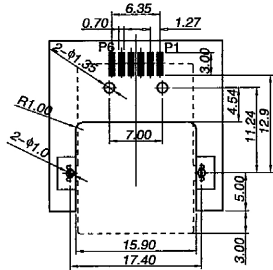
Recommend PCB Layout Jack Top View
