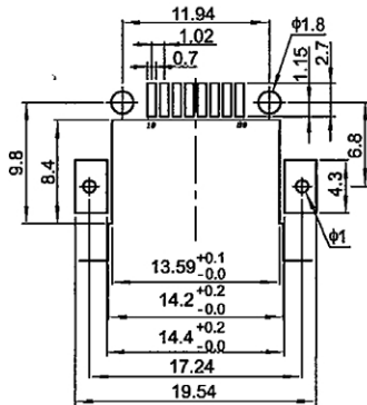
Recommend PCB Layout Jack Top View
