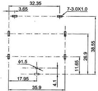
Recommend PCB Layout Jack Top View
