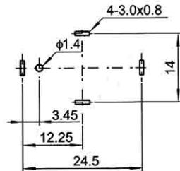
Recommend PCB Layout Jack Top View
