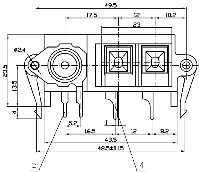
Dimensions of PC board holes (Commend)
