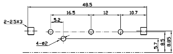
Dimensions of PC board holes (Commend)
