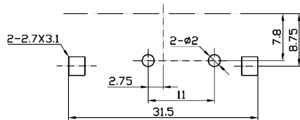
Dimensions of PC board holes (Commend) Bottom View ( t=1.6\text{mm} ) \odot
